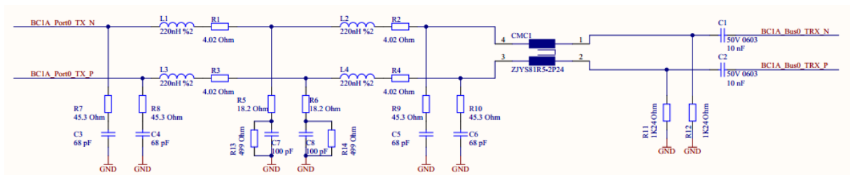
Figure 5-2: BR-Filter for HW v2.0
