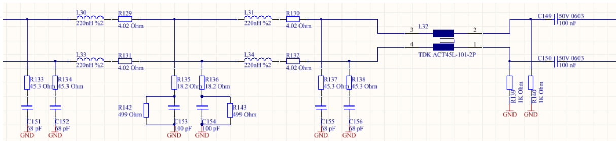
Figure 5-1: BR-Filter for HW v3.0 and v3.0a
